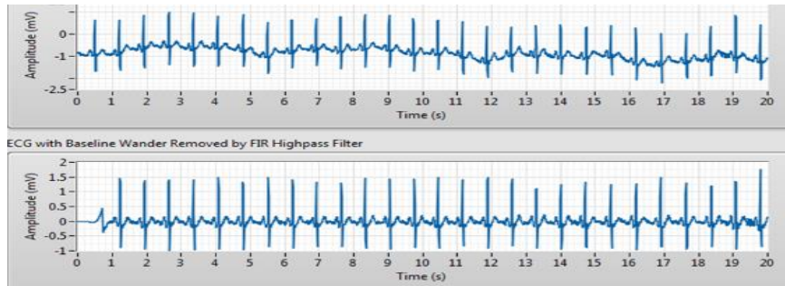
Figure 1: comparison between two electrocardiogram (ECG) signals before and after filtering
